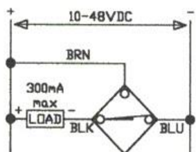
Cable - NPN/N.C. Wiring Diagram #4
