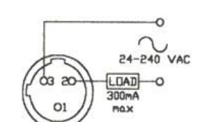
Cable - AC/N.O. Wiring Diagram #5
