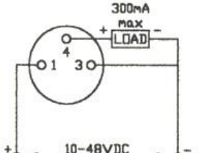
PICO - PNP Wiring Diagram #11
