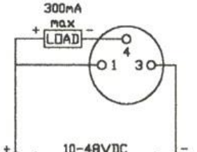
PICO - NPN Wiring Diagram #10
