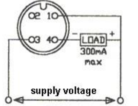
MICRO - NPN Wiring Diagram #8
